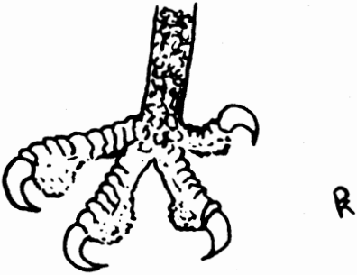
Prey-grasping Foot
