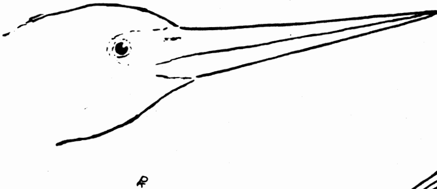
Fish Spear
