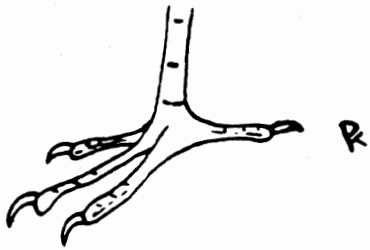
Perching Foot
