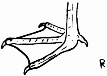
Swimming Foot
