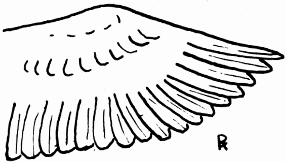
Generalized Wing
